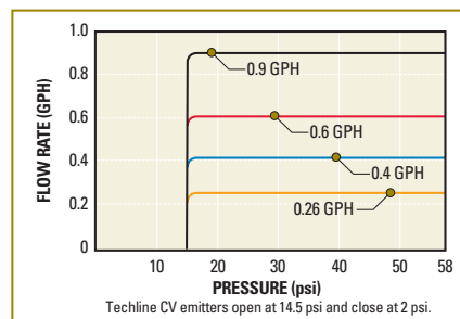
FLOW RATE VS. PRESSURE
